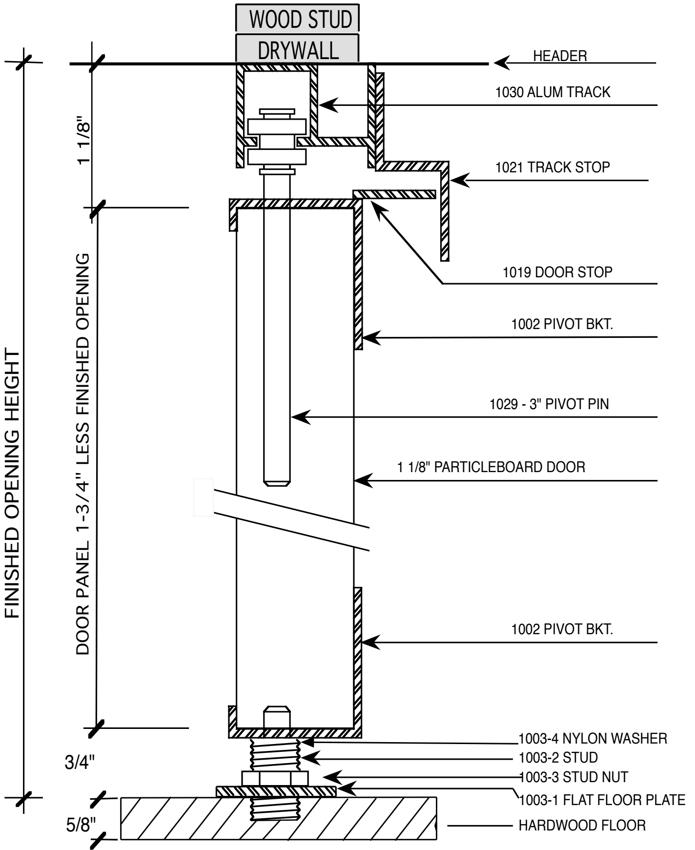
TYPICAL SECTION @ 1-1/8" BIFOLD DOOR THIS FLOOR PLATE IS USED FOR HARDWOOD & TILE CONDITIONS
