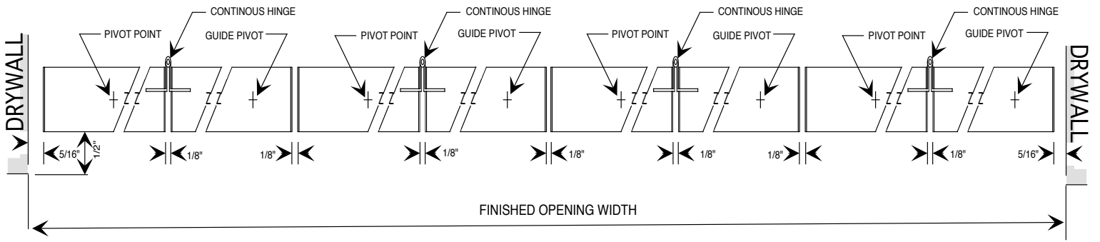
TYPICAL 8 PANEL BIFOLD DOOR CLEARANCES
